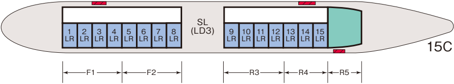
Lower Deck
